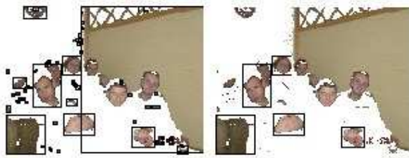
Fig. 4: An example of bad results of face detection performed in the 2D colour space: All found regions are shown on the left side of the figure and all kept regions are shown on the right side of the figure. The reason for bad performance is explained in the text.
